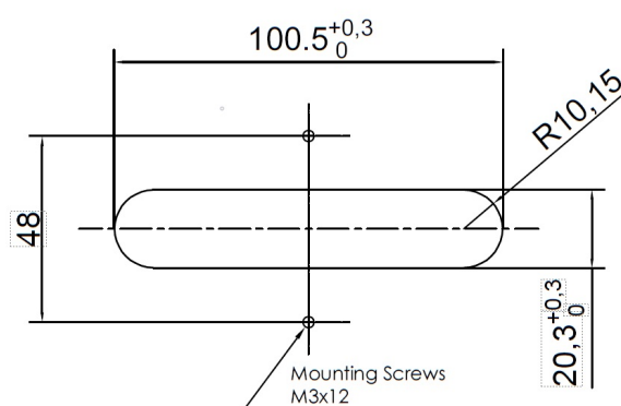
Mounting Diagram_Clip
